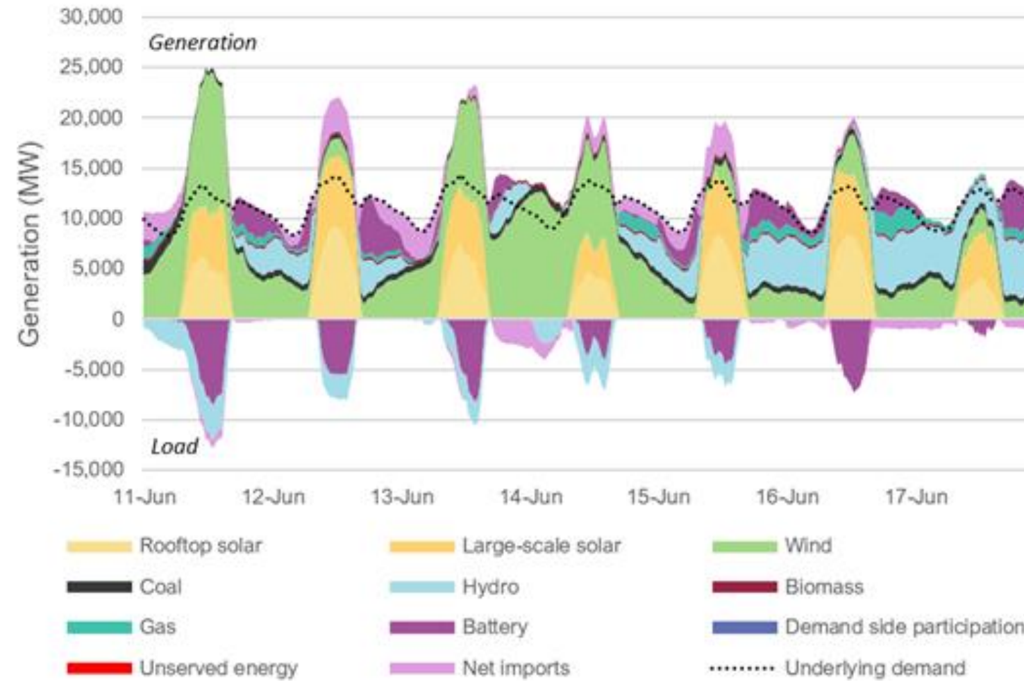
Typical weather conditions in June 2034-35
