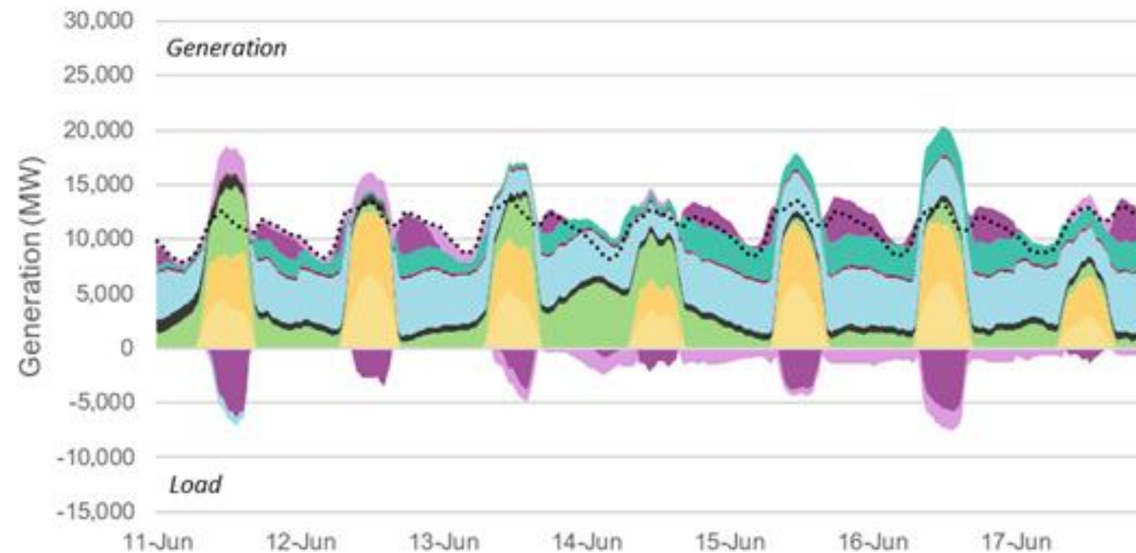
7-day VRE lull in June 2034-35
